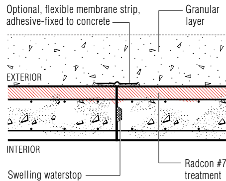
DETAIL TPJ2 CONSTRUCTION JOINT
