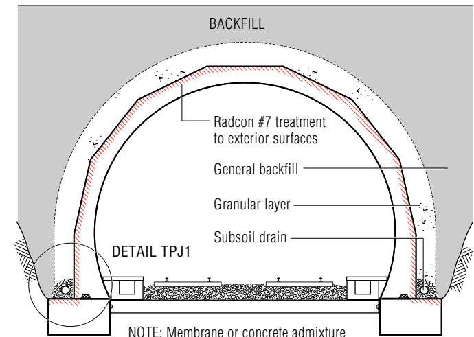
DETAIL TPJ1
