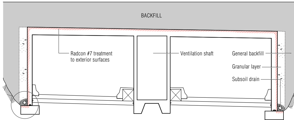
DETAIL TPJ1
